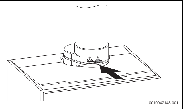
Afb. 35 Rookgasmeetnippel
