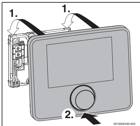
Afb. 8 Bedieningsunit inhangen
