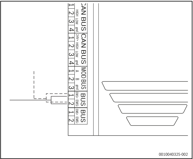
Afb. 38 Verbinding EMS
