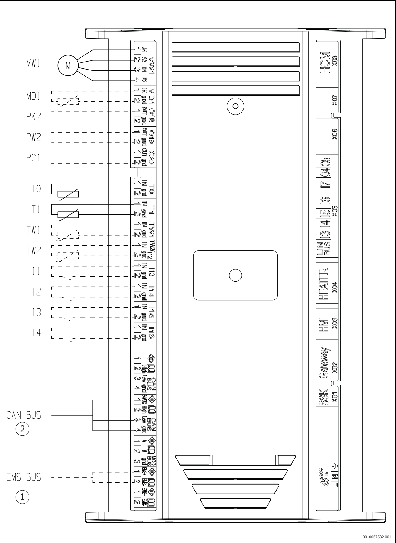
Fig. 70 XCU-THH de raccordement
