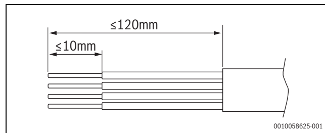
Afb. 32 Strippen CAN BUS
