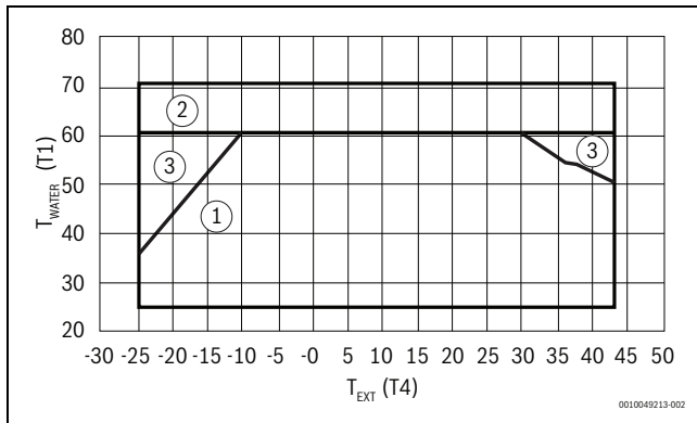
Afb. 10 CS2000AWF 18-30 R-T
