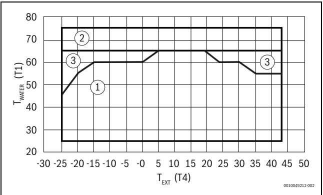
Afb. 9 CS2000AWF 4-6 R-S, CS2000AWF 8-10 R-S, CS2000AWF 12-16 R-S/T
