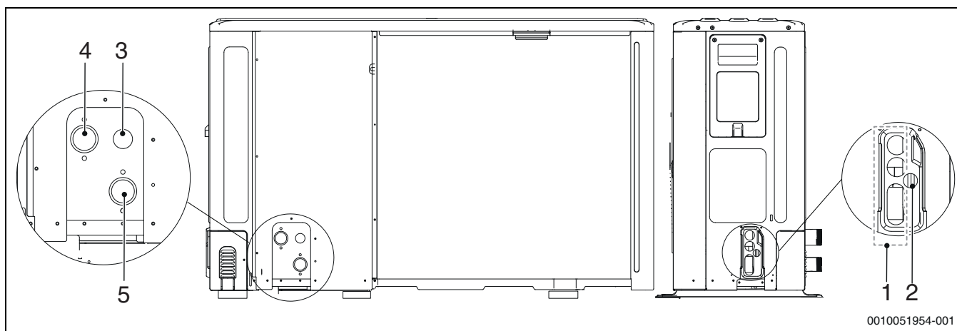
Afb. 65 Afmetingen CS2000AWF 8 R-S tot CS2000AWF 16 R-S/CS2000AWF 16 R-T
