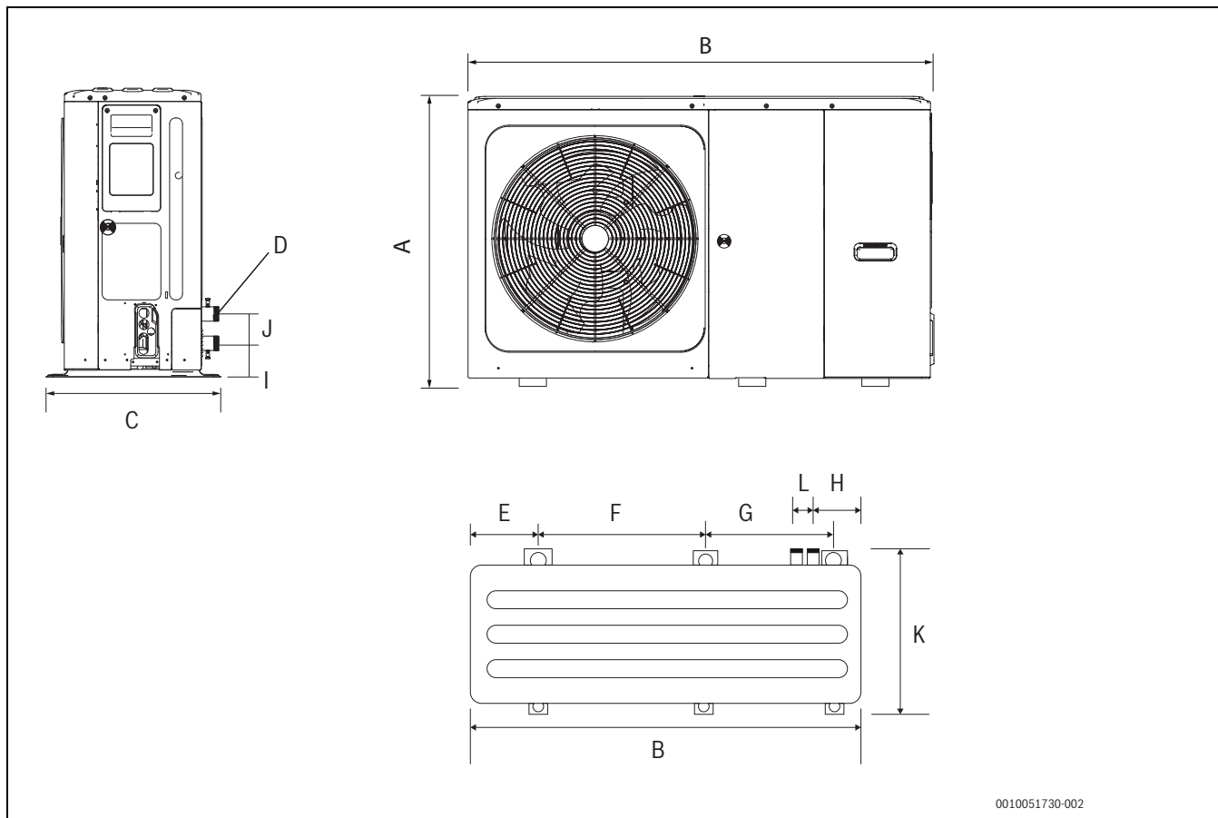
Afb. 33 Modellen CS2000AWF 8 R-S tot CS2000AWF 16 R-S/CS2000AWF 16 R-T
