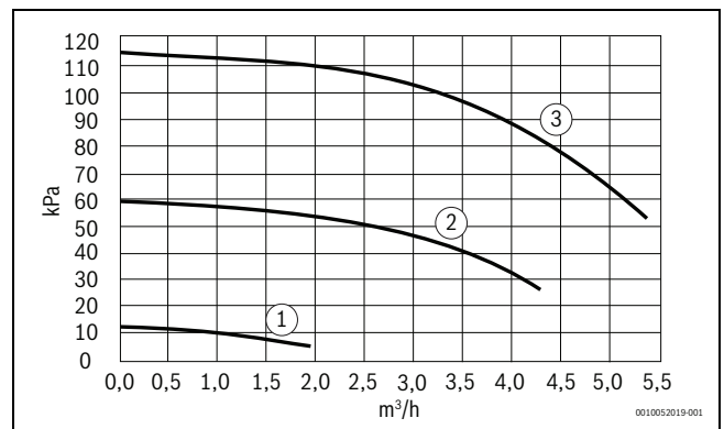
Afb. 14 CS2000AWF 18-30 R-T
