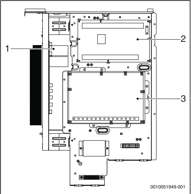
Afb. 63 Afmetingen CS2000AWF 18 R-T tot CS2000AWF 16 R-S/CS2000AWF 30 R-T
