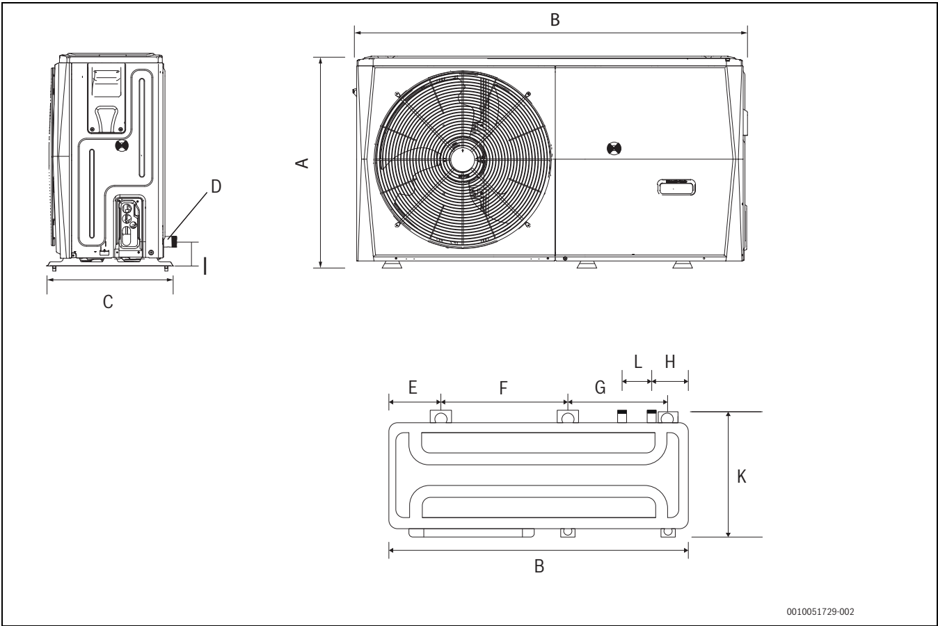
Afb. 32 Modellen CS2000AWF 4 R-S tot CS2000AWF 6 R-S
