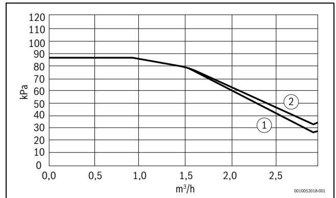
Afb. 13 CS2000AWF 4-6 R-S
