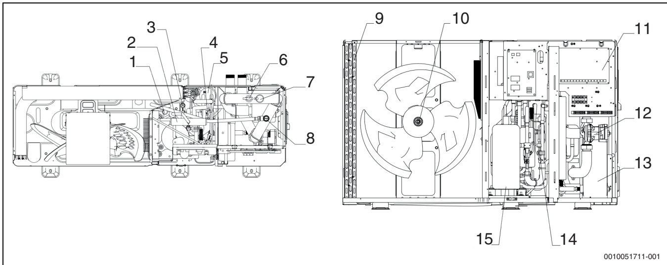
Afb. 4 Afmetingen CS2000AWF 12 R-S/CS2000AWF 12 R-T tot CS2000AWF 16 R-S/CS2000AWF 16 R-T
