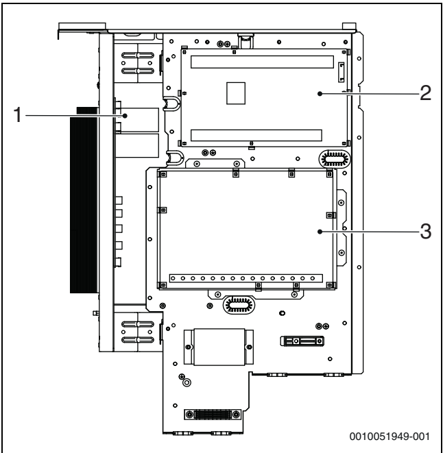
Afb. 62 Afmetingen CS2000AWF 4 R-S tot CS2000AWF 16 R-S/CS2000AWF 16 R-T
