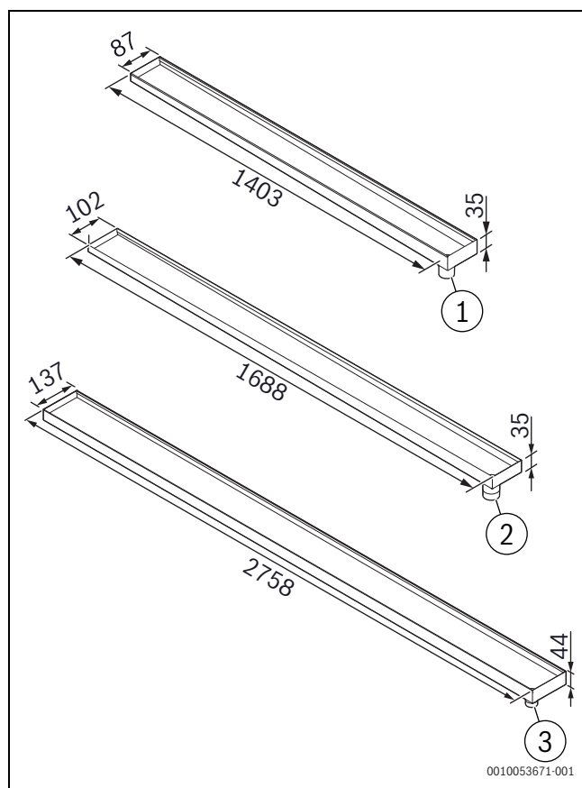
Afb. 13 Condensbak chassis 1-4
