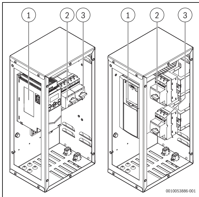
SI.41 Inverter pumpe AWP65 – AWP89
