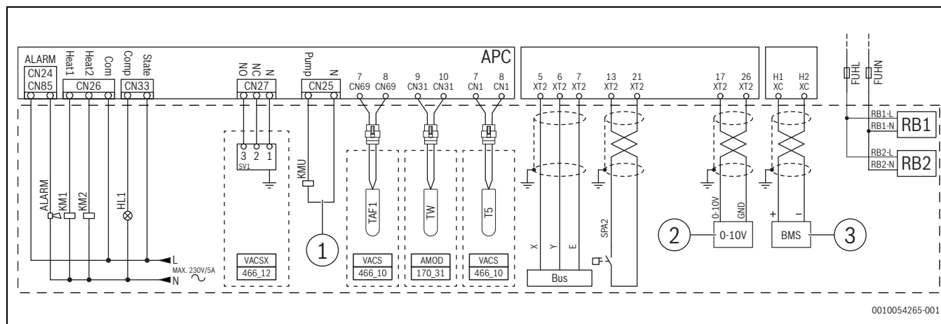
SI.29 AWP16 – AWP24 (≥ 06.2024)
