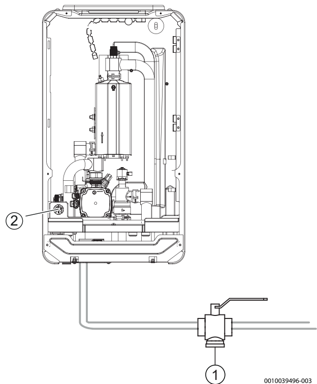
Afb. 15 Binnenunit Compress 5800i 12 E
