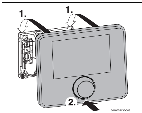
Afb. 8 Bedieningsunit inhangen
